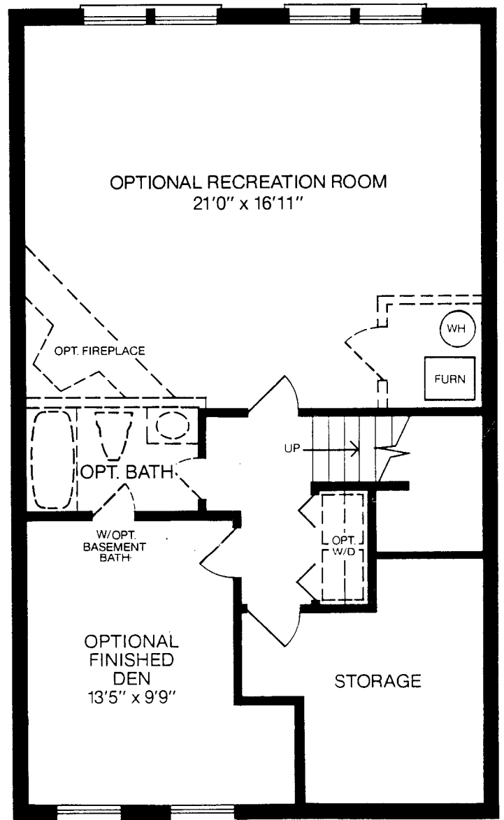
ENGLISH BASEMENT PLAN
